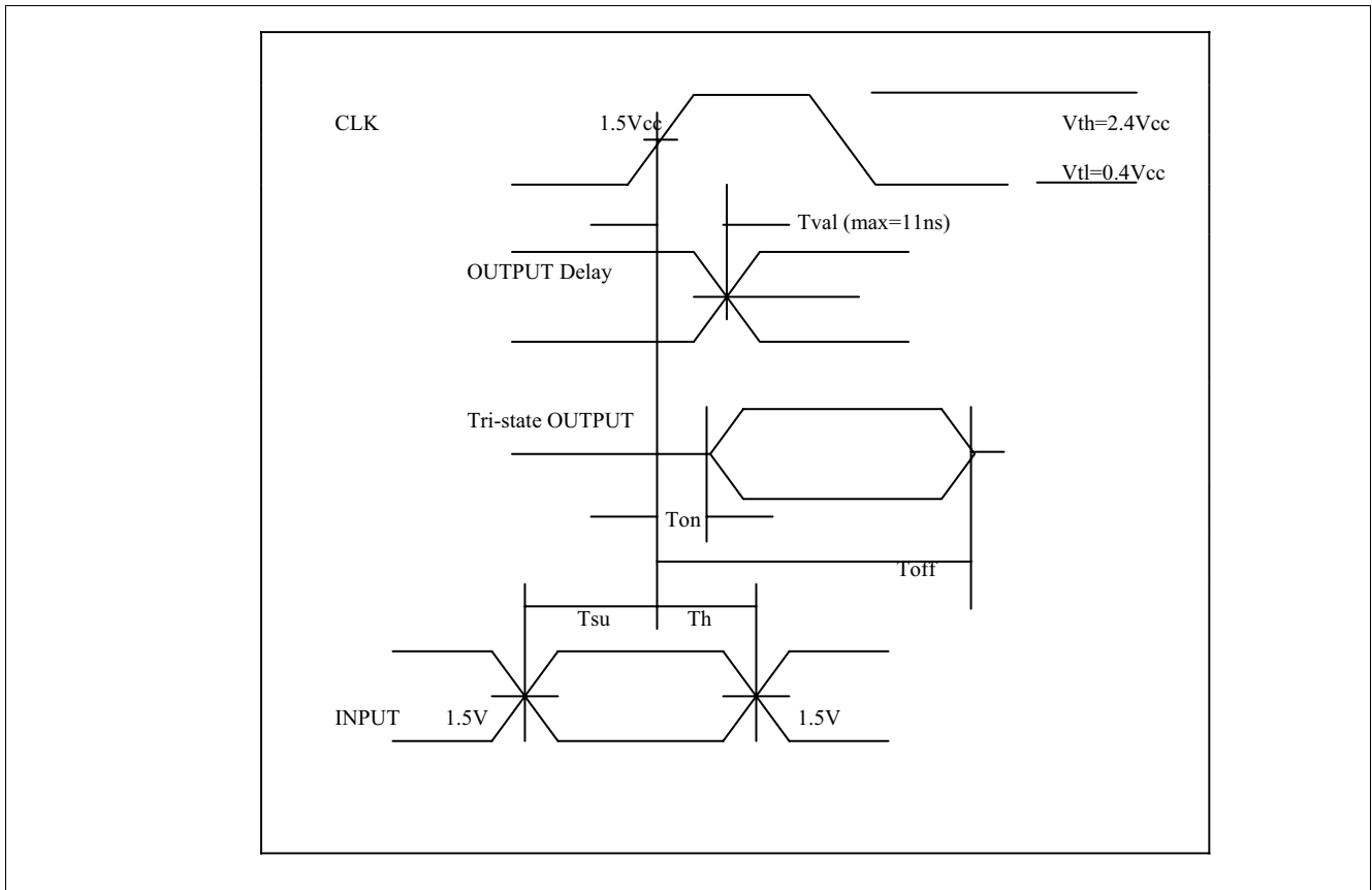
Figure 18 PCI Timings
